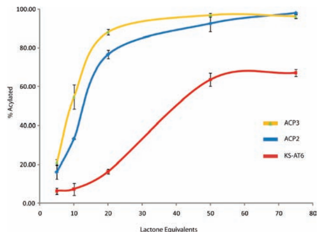
Figure 2. Saturation curves as determined by tandem proteolysis-mass spectrometry for ACP3 (yellow), ACP2 (blue), and KS-AT6 (red) with compound 1 . Equivalents of lactone are per protein molecule. Each data point is the average of three experiments. Standard deviations are shown as black error bars. Lines are added for clarity.
